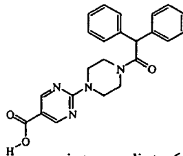
intermediate 6
